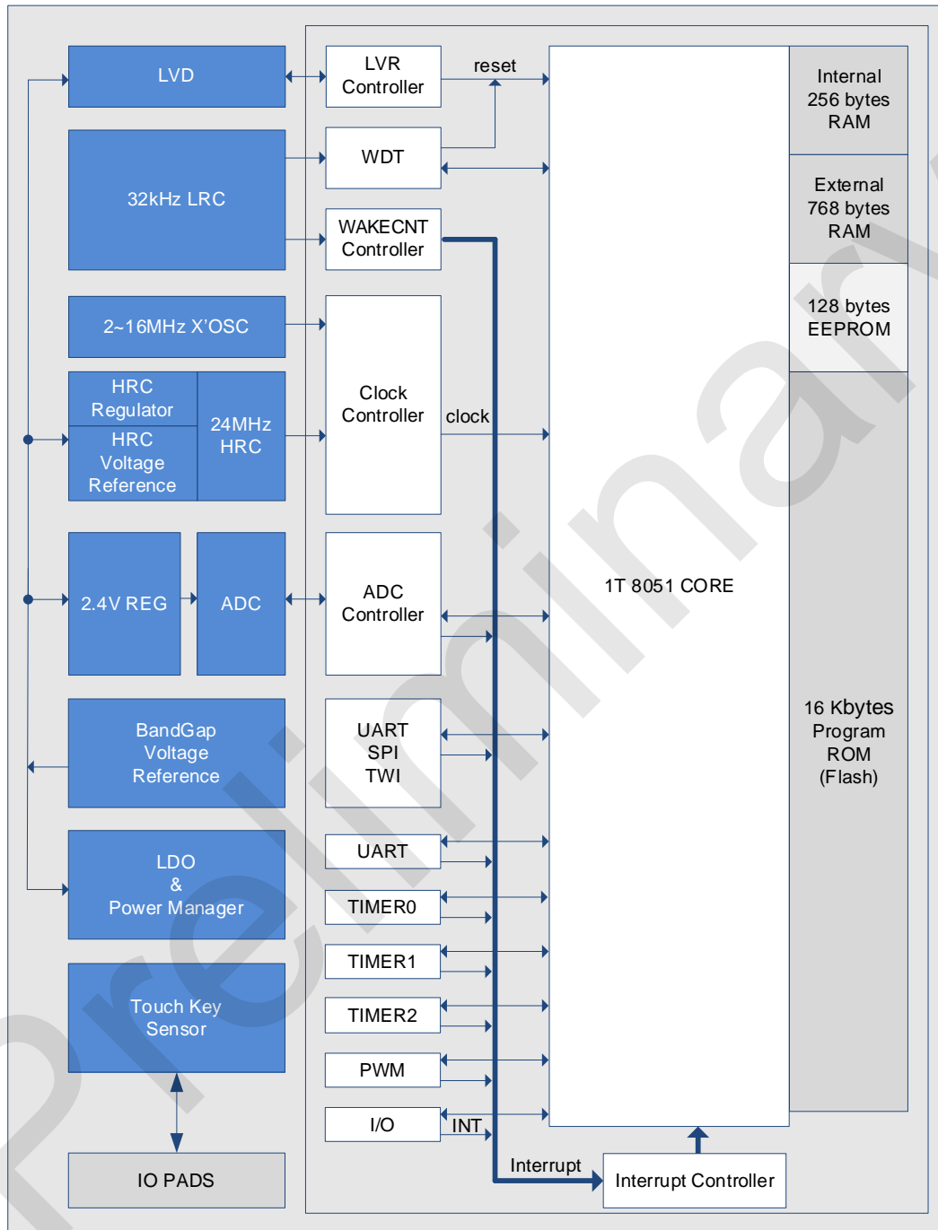
SC92F841XB BLOCK DIAGRAM
